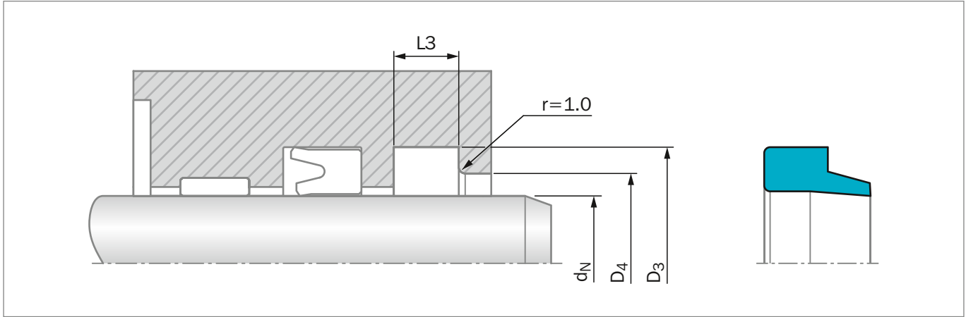
Figure 204: Installation Drawing
