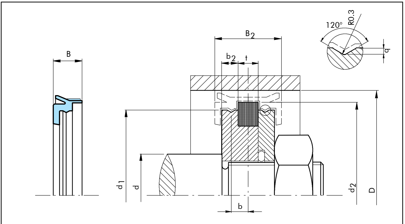
Figure 9 Installation drawing
