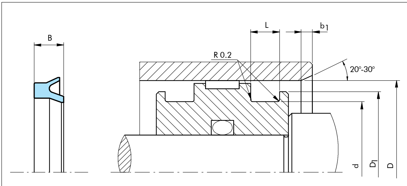
Figure 7 Installation drawing
